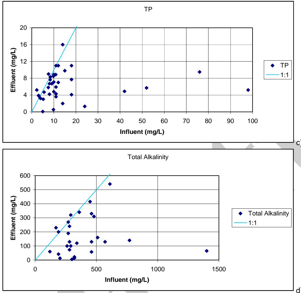
Figure 4. Influent and effluent concentrations for composite samples, where both were sampled during the same sampling event. Influent excludes samples with high solids, tap water and recirculation systems. a) cBOD5 and TSS; b) TN; c) TP; d) Total Alkalinity.
