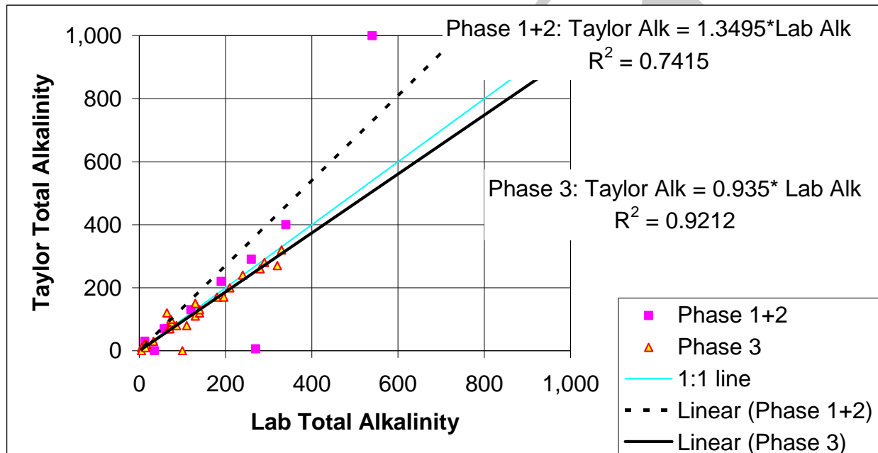
Figure 6. Illustration of the relationship between total alkalinity measurements in the laboratory and measurements using a Taylor kit.
