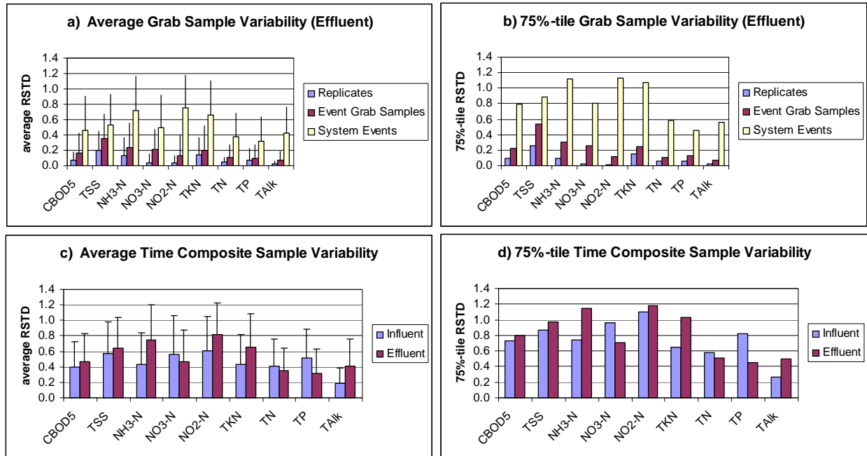
Figure 3. Comparisons of variability between samples. a) average relative standard deviations (+ one standard deviation) of replicates, grab samples during an event, and events for a system; b) 75%-tile of the relative standard deviations of replicates, grab samples during and event, and events for a system; c) average relative standard deviations (+one standard deviation) for influent and effluent time composite samples between events for a system; d) 75%-tile for influent and effluent relative standard deviations between events for a system
