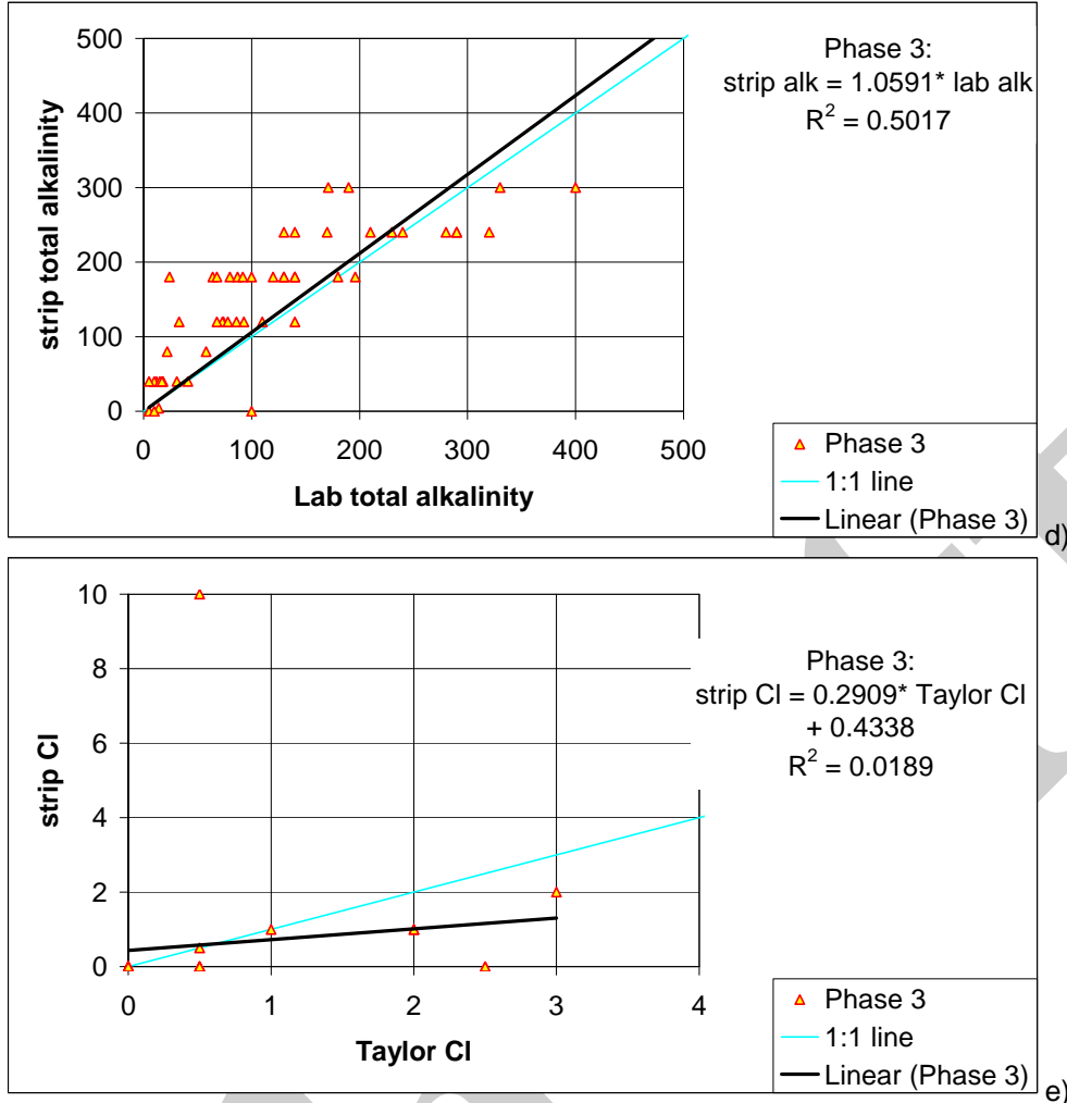
Figure 7. Relationships between other measures of concentrations and results of test strip measurements: a) ortho-phosphorus vs. lab TP b) nitrate vs lab nitrate-N c) nitrite vs lab nitrite d) alkalinity vs. lab total alkalinity e) chlorine vs Taylor chlorine
